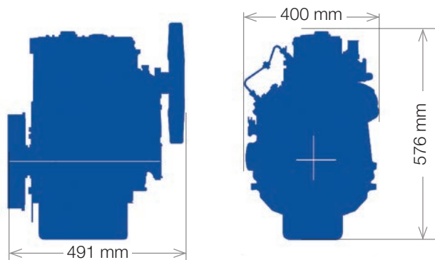
Engine package weights and dimensions
